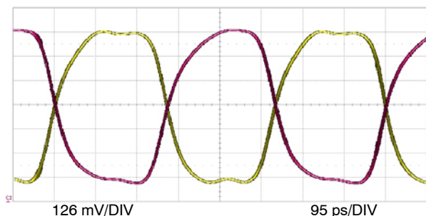
Figure 4. Typical Output Waveform at 2 GHz ( V_{INPP} = 175 \text{ mV} , V_{CC} = 2.38 \text{ V} )
