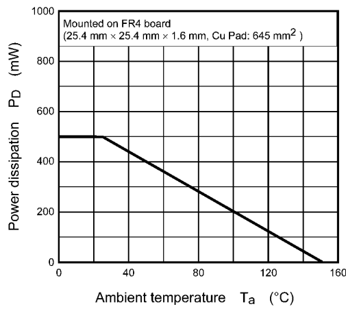
Fig. 8.11 P_D - T_a
