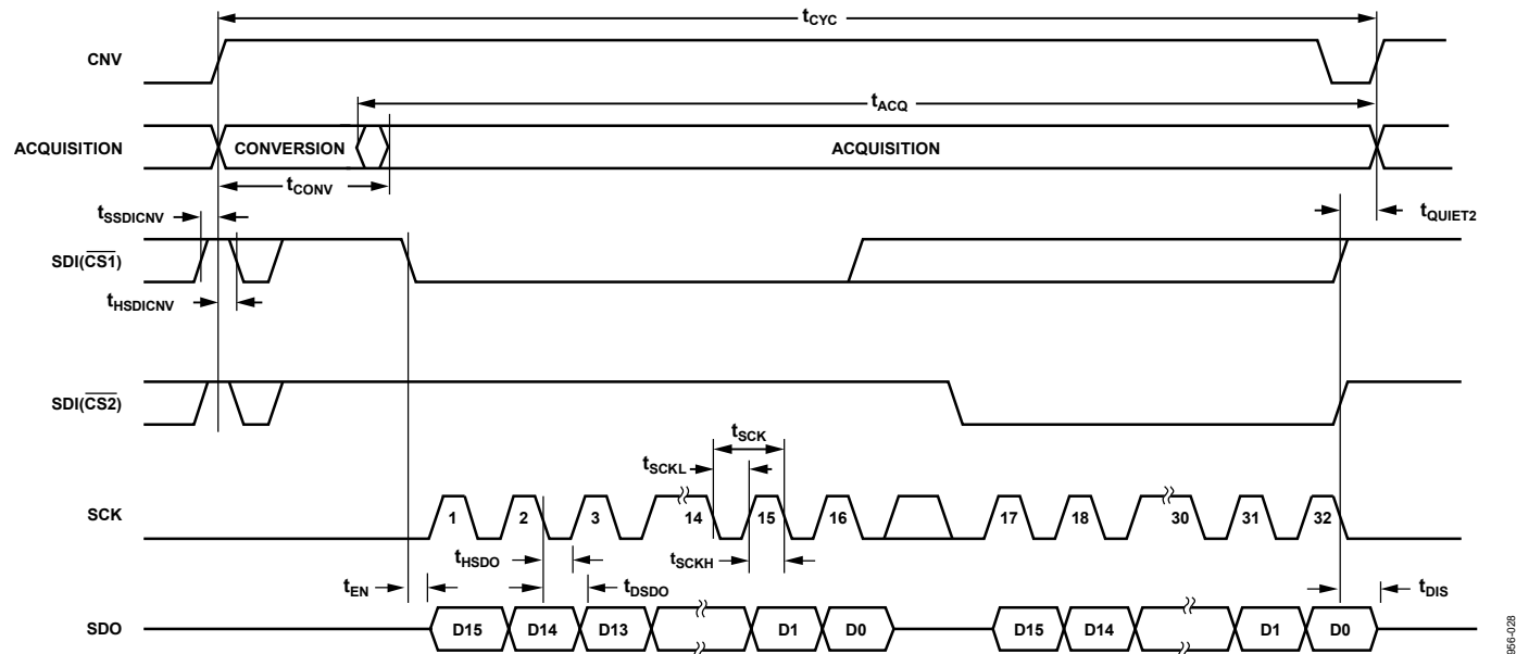
Figure 59. \overline{\text{CS}} Mode, 4-Wire Without Busy Indicator Serial Interface Timing Diagram (Status Bits Not Shown)
