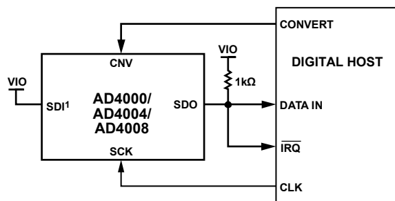
Figure 54. CS Mode, 3-Wire with Busy Indicator Connection Diagram
