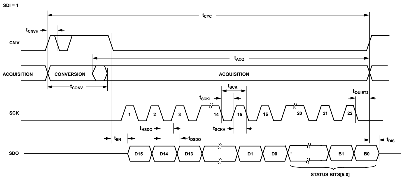
Figure 49. \overline{\text{CS}} Mode, 3-Wire Without Busy Indicator Serial Interface Timing Diagram, Including Status Bits
