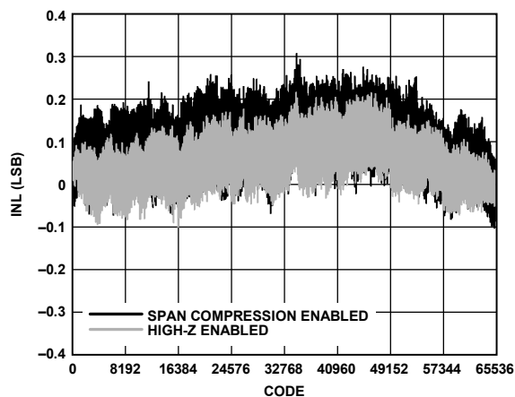
Figure 7. INL vs. Code for High-Z and Span Compression Modes Enabled, V_{REF} = 5\text{ V}
