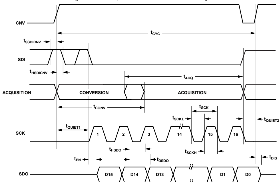
Figure 57. \overline{\text{CS}} Mode, 4-Wire Turbo Mode Timing Diagram (Status Bits Not Shown)
