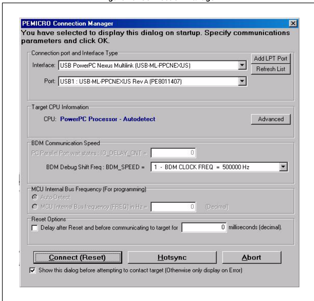
Figure 19. Connection manager
