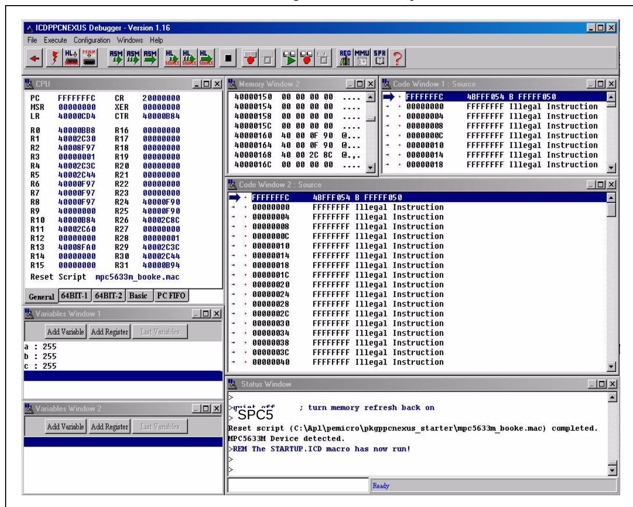
Figure 20. Default layout
