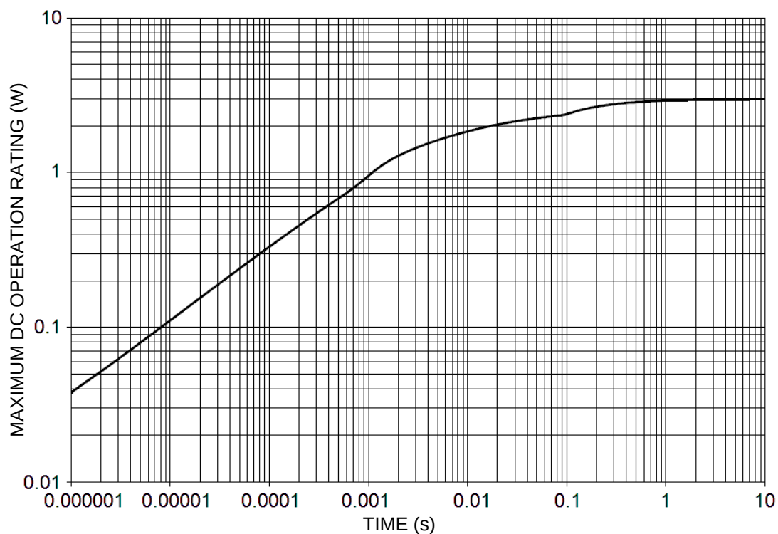
FIGURE 2 Thermal Impedance
