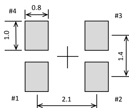
[ 8 ] Recommended foot print unit:mm
