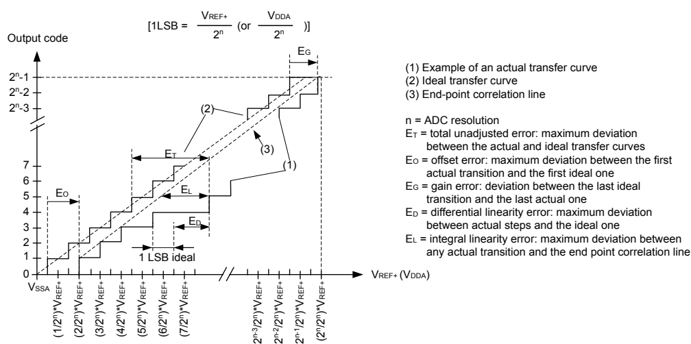
Figure 32. ADC accuracy characteristics
