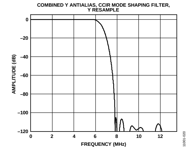
Figure 19. Combined Y Antialias, CCIR Mode Shaping Filter
