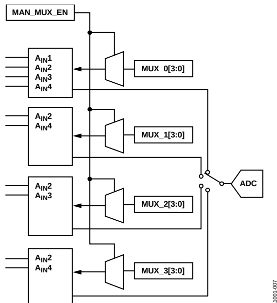
Figure 8. Manual Muxing
