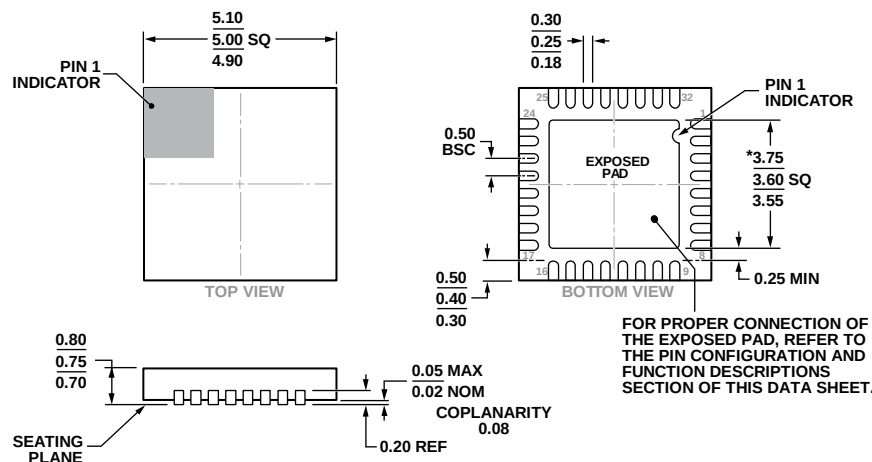
Figure 51. 32-Lead Lead Frame Chip Scale Package [LFCSP_WQ] 5 mm × 5 mm Body, Very Very Thin Quad (CP-32-12)
