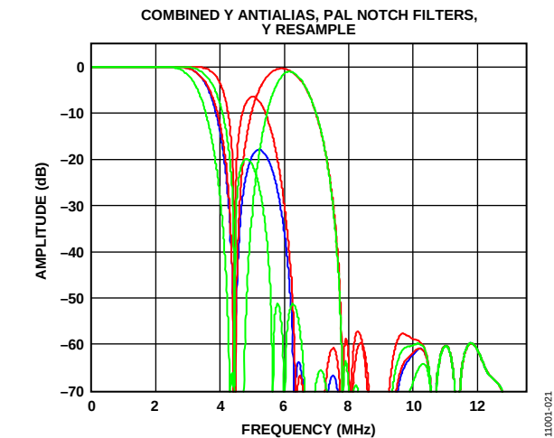
Figure 20. Combined Y Antialias, PAL Notch Filters
