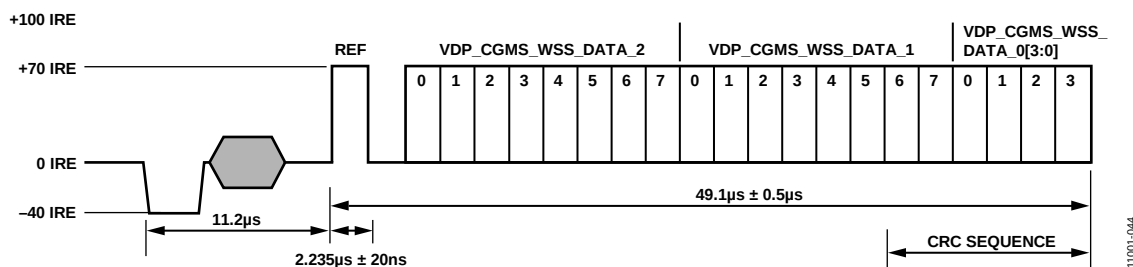
Figure 43. CGMS Waveform
