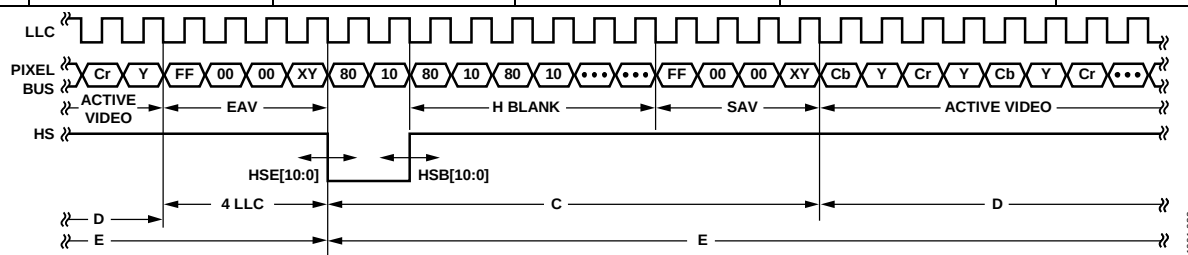
Figure 31. HSYNC Timing
