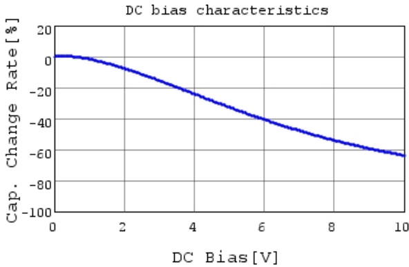
GRM033R61A473KE84 C-DC bias capchange, 25.0c
