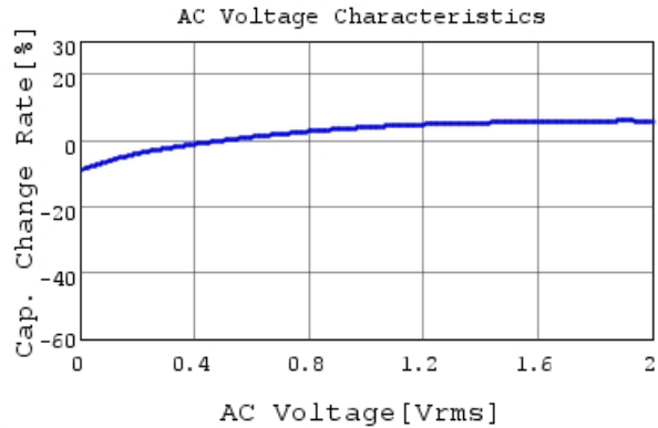
GRM033R61A473KE84 C-AC Voltage capchange, Dc
