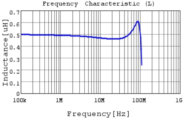
DFE201612PD-R47M L
