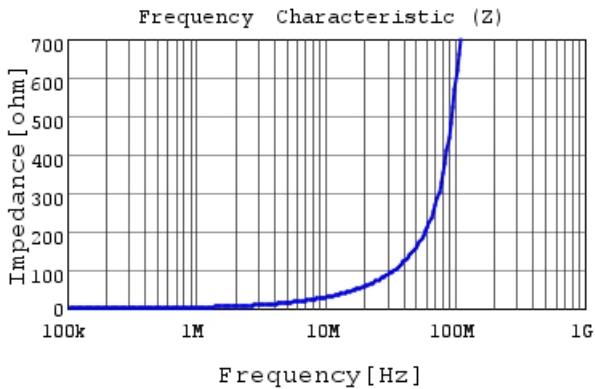
DFE201612PD-R47M |Z|
