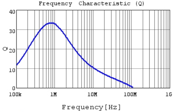
DFE201612PD-R47M Q
