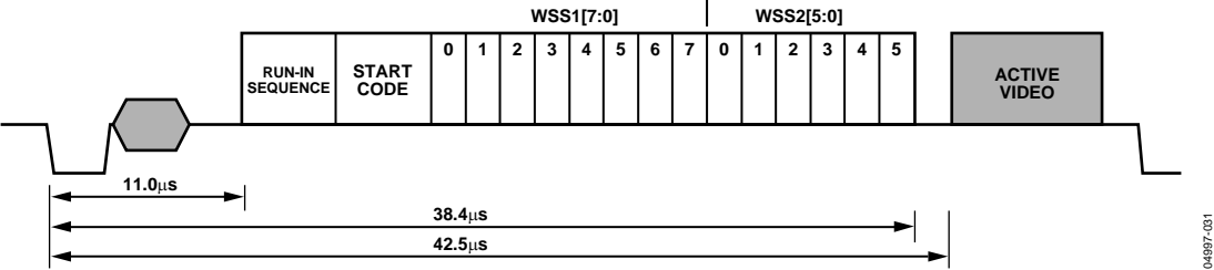
Figure 31. WSS Data Extraction
