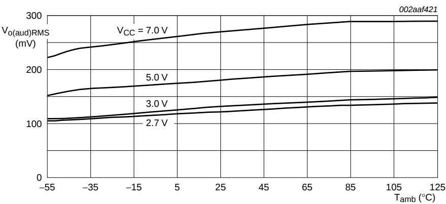
Fig 15. RMS audio output voltage versus ambient temperature
