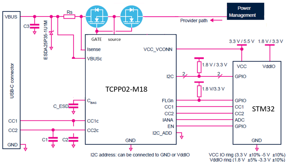
Figure 4. Application block diagram example
