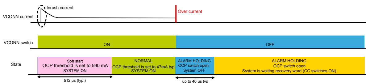
Figure 10. V CONN OCP chronograms
