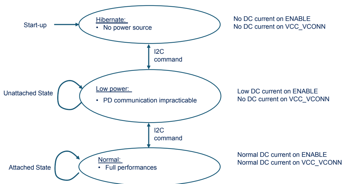
Figure 6. Power modes process
