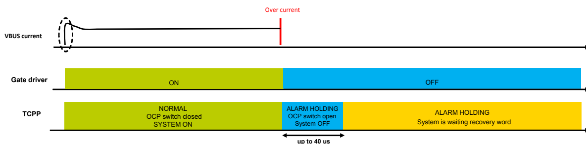
Figure 9. Typical chronograms of TCPP02-M18 VBUS OCP
