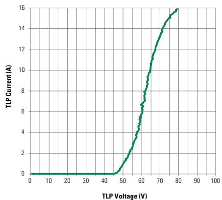
SPHV36-C Transmission Line Pulsing(TLP) Plot
