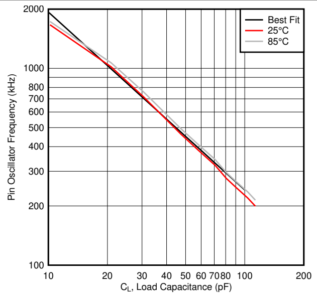
Figure 8-13. Typical Oscillation Frequency vs Load Capacitance
