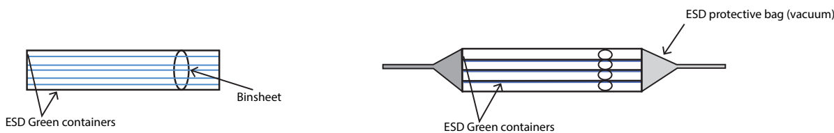
Fig 14. Example of the packaging for LUXEON FlipChip Royal Blue.
