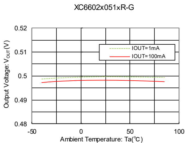
(7) Output Voltage vs. Ambient Temperature
