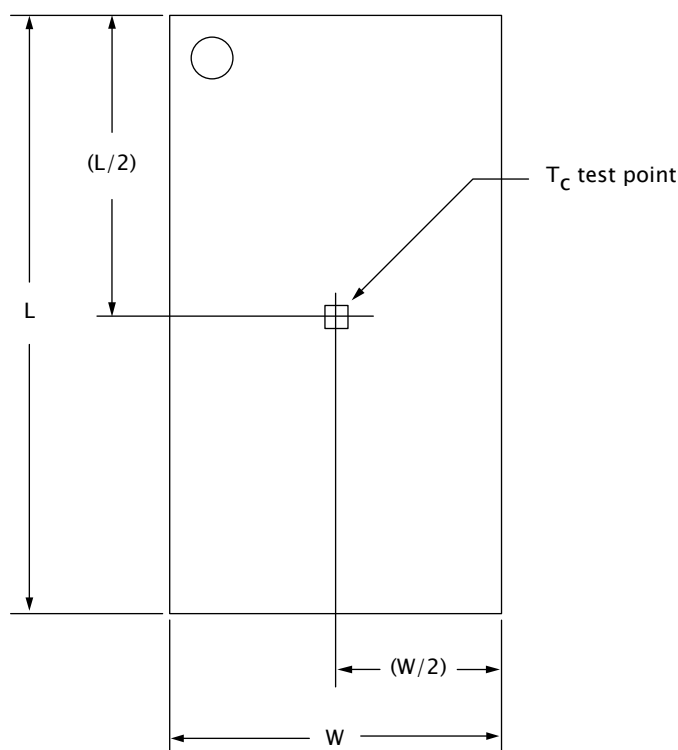
Figure 5: Thermal Measurement Point
