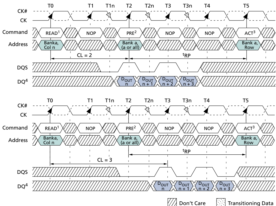
Figure 37: READ-to-PRECHARGE
