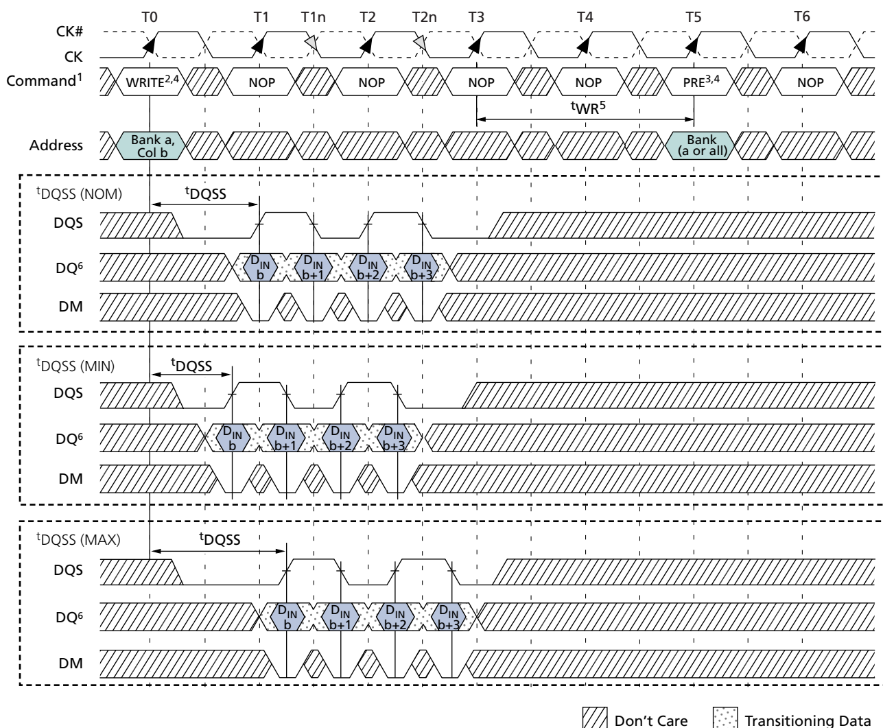
Figure 50: WRITE-to-PRECHARGE – Uninterrupting
