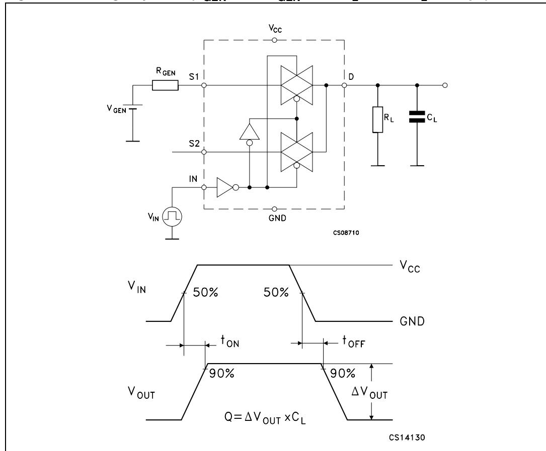
Figure 10. Charge injection ( V_{GEN} = 0 V, R_{GEN} = 0 \Omega , R_L = 1 M \Omega , C_L = 100 pF)
