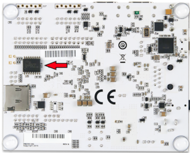
Figure 4.1. Arty Z7 Flash IC Location
