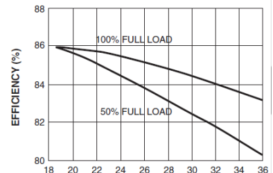
24 VOLT EFFICIENCY Vs. LINE INPUT VOLTAGE
