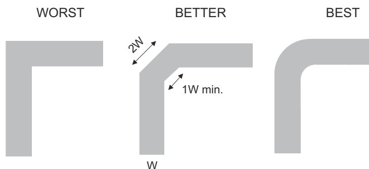
Figure 11-1. Trace Example
