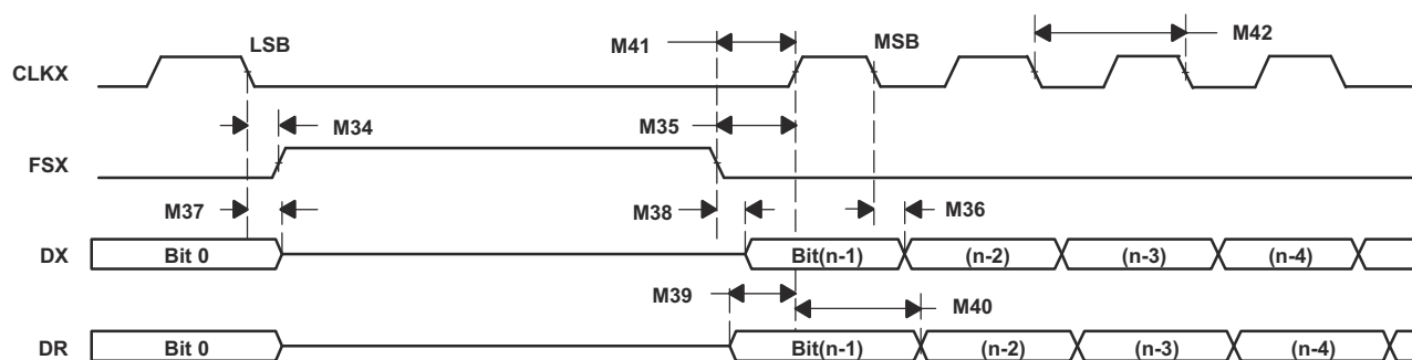
Figure 6-72. McBSP Timing as SPI Master or Slave: CLKSTP = 11b, CLKXP = 0
