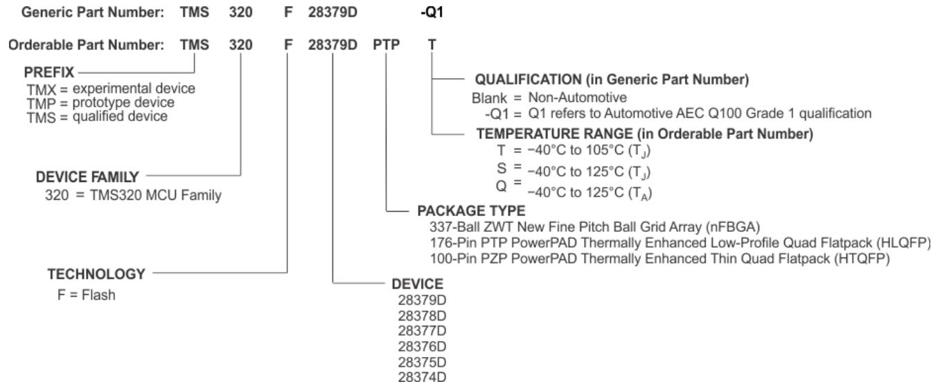
Figure 9-1. Device Nomenclature
