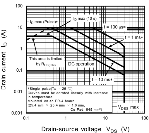
Fig. 8.1.12 Safe Operating Area
