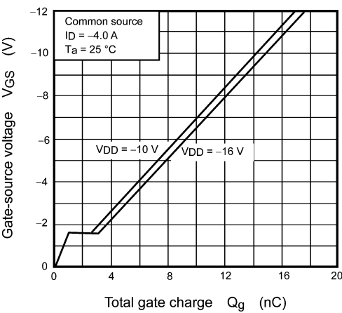
Fig. 8.2.10 Dynamic Input Characteristics
