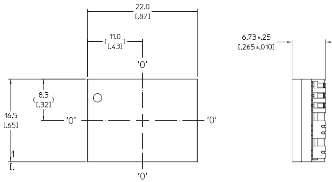
TOP VIEW (COMPONENT SIDE)
