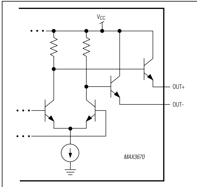
Figure 2. Output Interface
