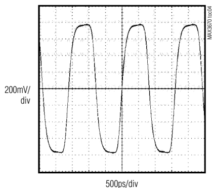
622MHz CLOCK OUTPUT (DIFFERENTIAL OUTPUT)
