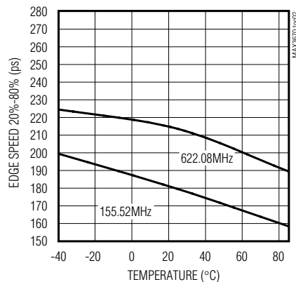
EDGE SPEED vs. TEMPERATURE
