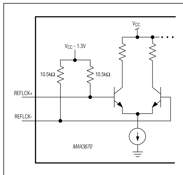
Figure 1. Input Interface
