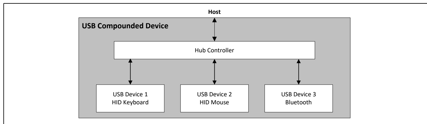
Figure 14. USB Compounded Device Configuration
