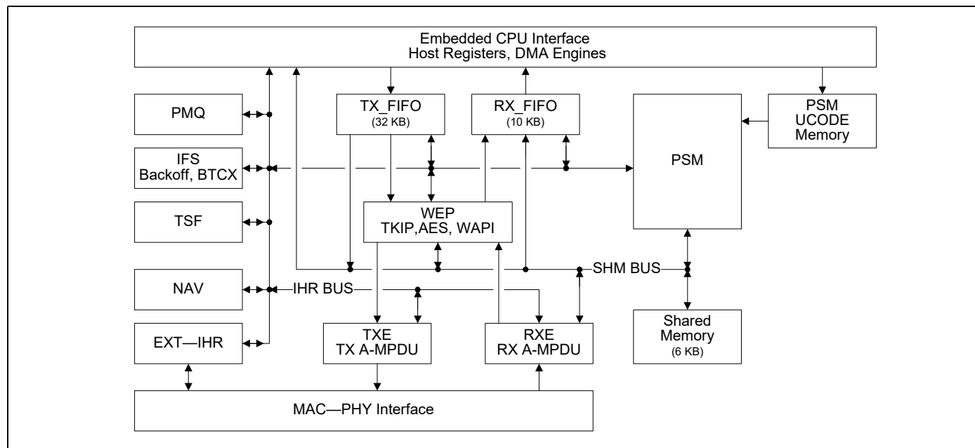
Figure 20. WLAN MAC Architecture
