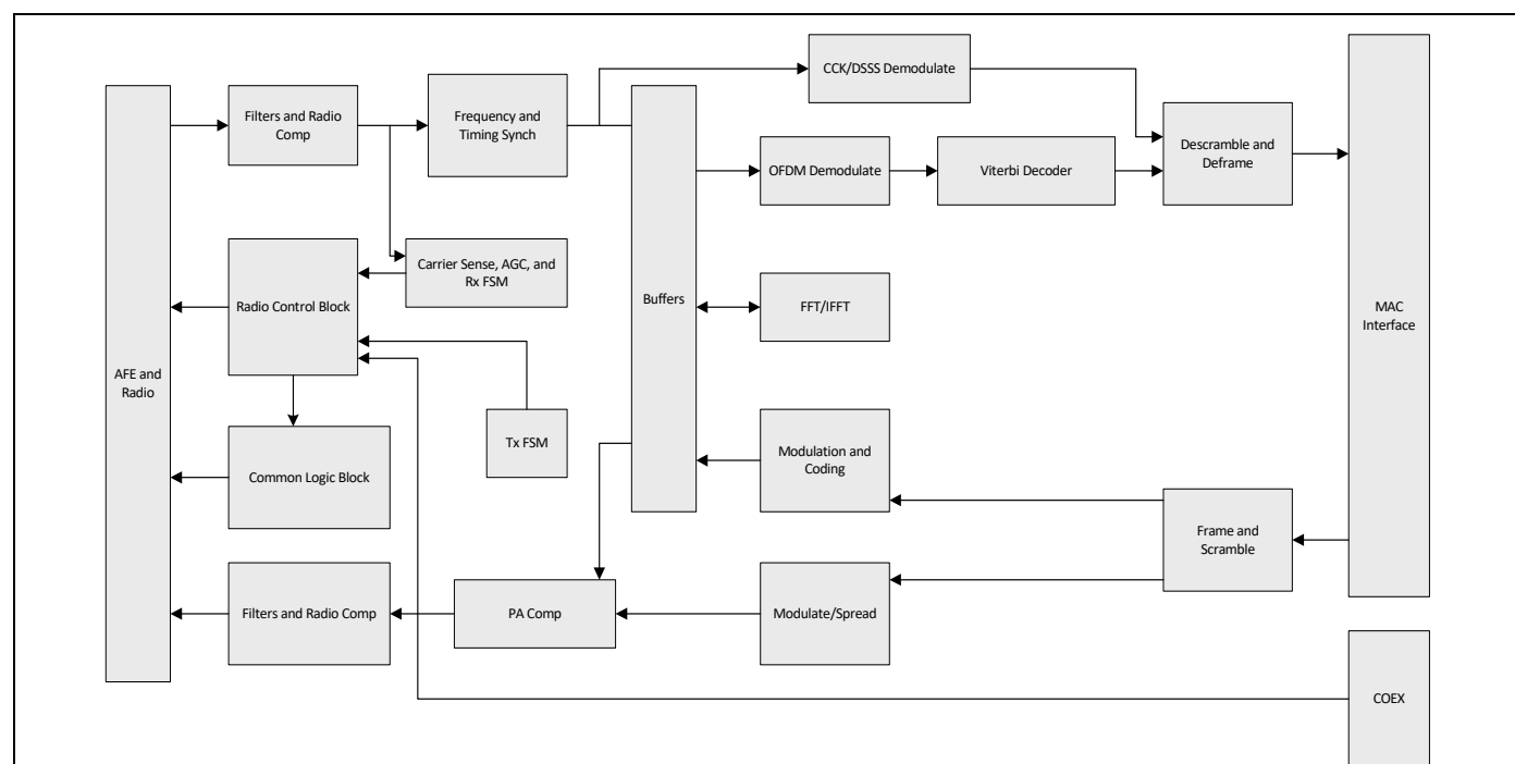
Figure 21. WLAN PHY Block Diagram
