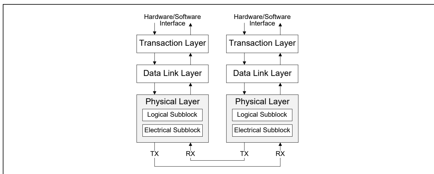
Figure 19. PCI Express Layer Model
