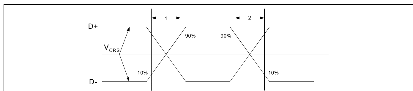
Figure 15. USB Full-Speed Timing
