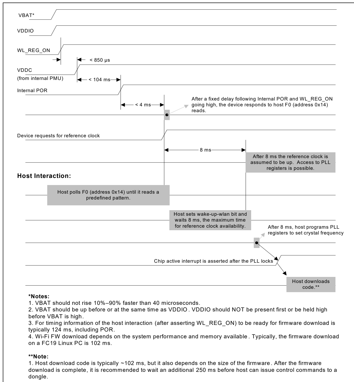
Figure 30. WLAN Boot Sequence
