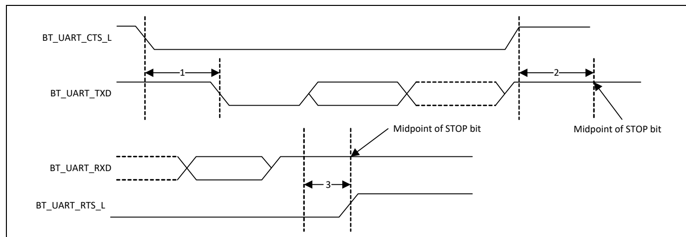
Figure 16. UART Timing
