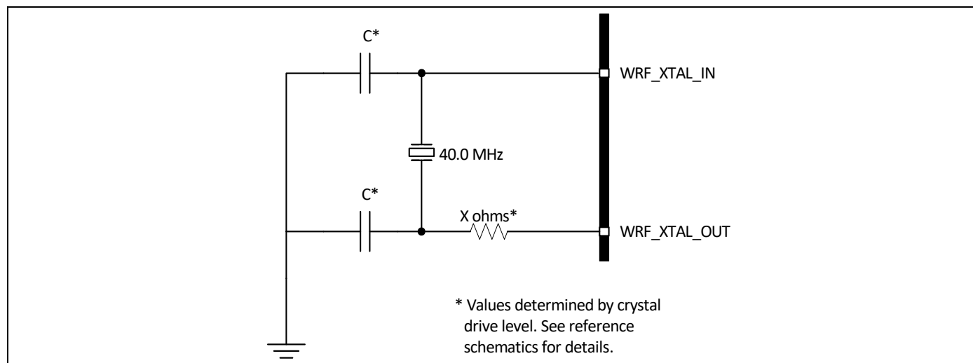
Figure 4. Recommended Oscillator Configuration
