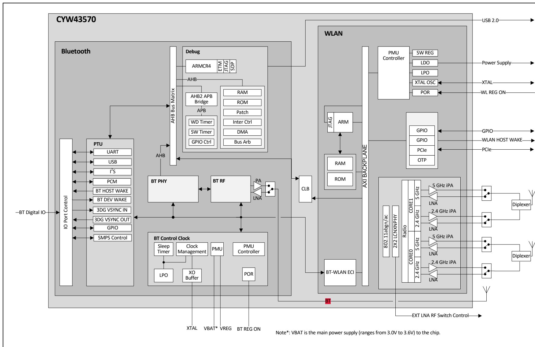
Figure 2. CYW43570 Block Diagram
