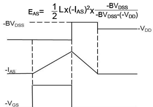
Figure 10. EAS Waveform
