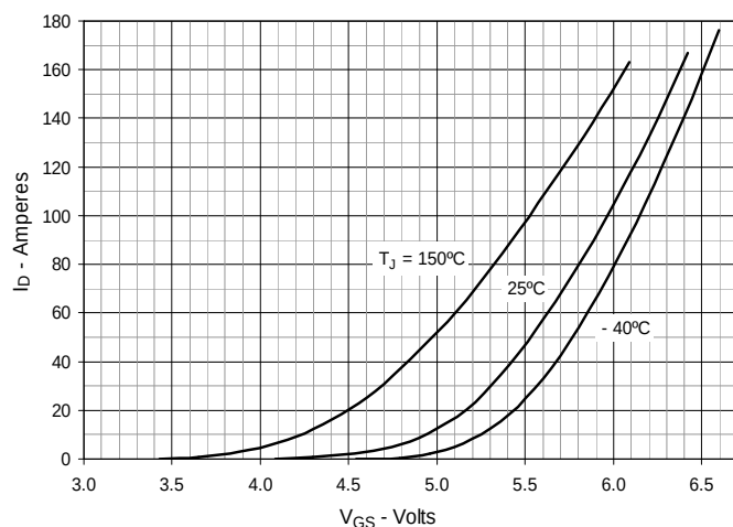
Fig. 7. Input Admittance
