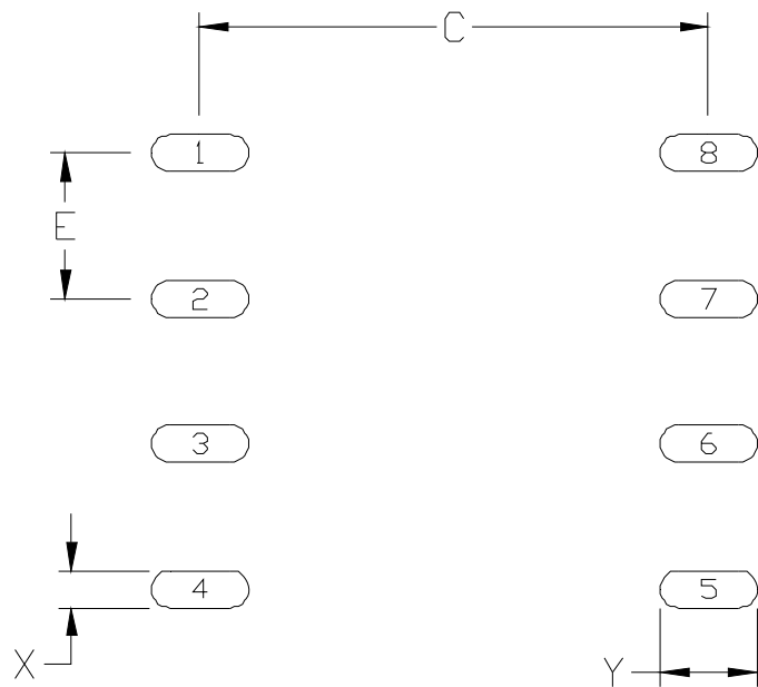
Figure 19. DIP8 Land Pattern
