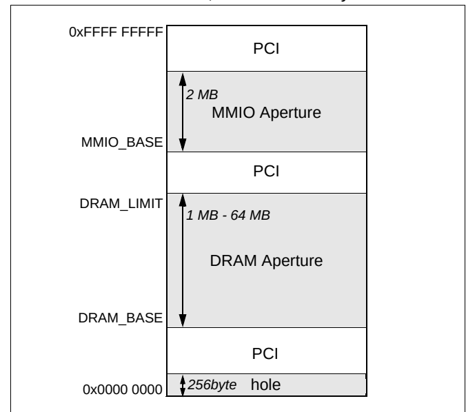
Figure 3-4. PN1300 memory map.
