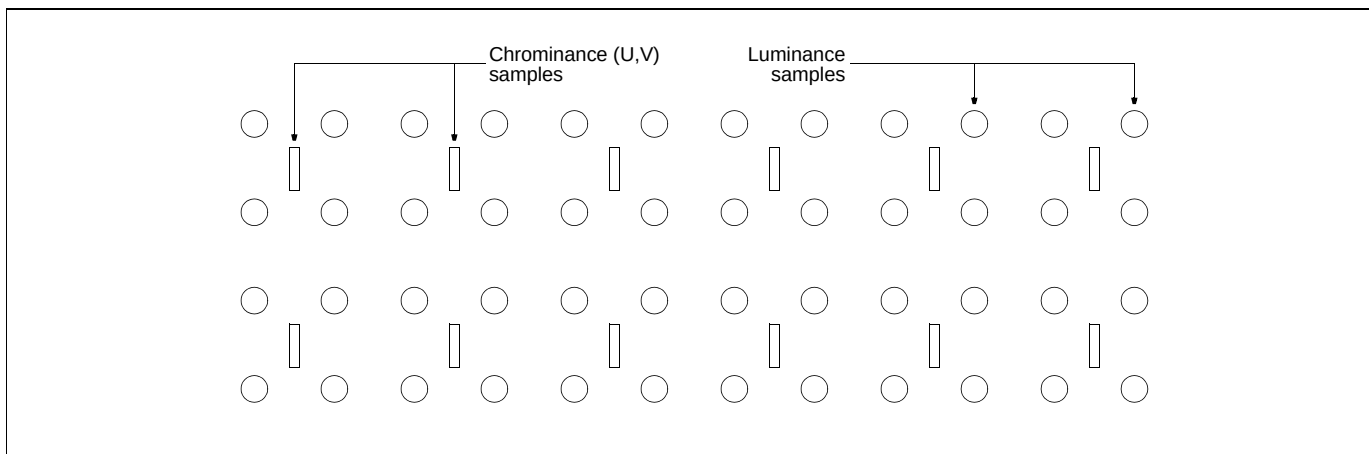
Figure 7-21. YUV 4:2:0 format.
