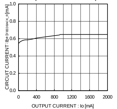
Fig.9 Circuit Current ( I_{FEEDBACK\_R} \approx 75\mu\text{A} )
