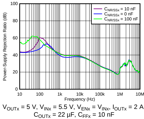
Figure 1. Power-Supply Rejection Ratio vs Frequency and C_{\text{NR/SSx}}
