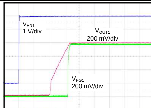
Figure 40. Start-Up ( \text{SS\_CTRLX} = \text{GND} , C_{\text{NR/SSX}} = 0\text{ nF} )
