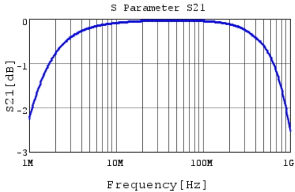
DE1E3KX222MA4BN01F S21 DC0V, 20degC
