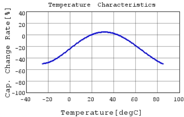
DE1E3KX222MA4BN01F C-Temp. capchange, DC0V,
