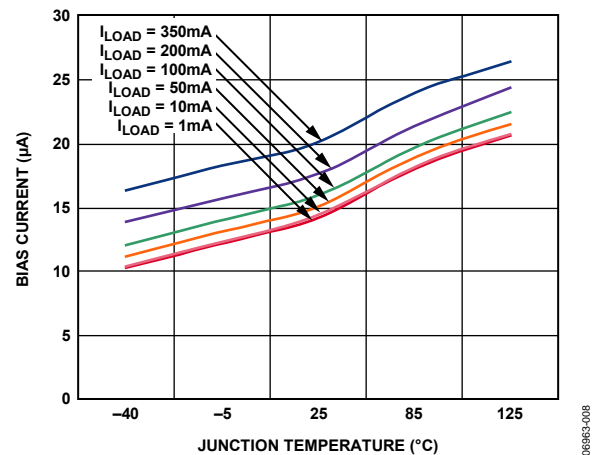
Figure 8. Bias Current vs. Junction Temperature
