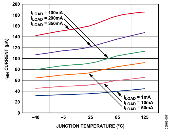
Figure 7. I_{VIN} Current vs. Junction Temperature
