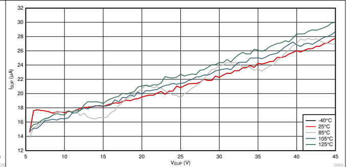
Figure 7-2. I_{SUP} vs V_{SUP} Across Temperature
