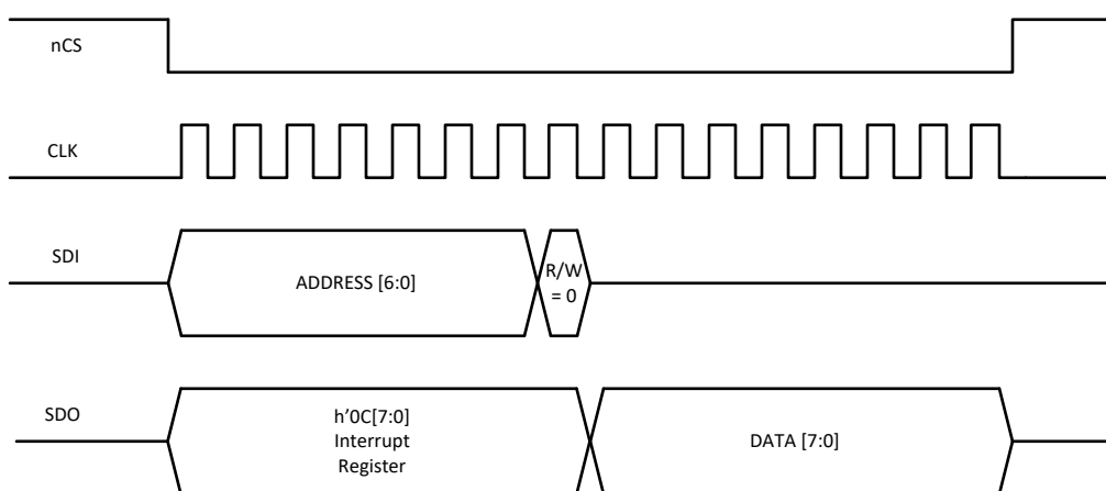
Figure 9-12. SPI Read
