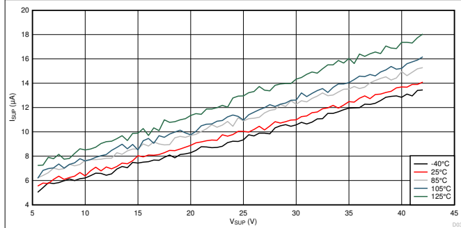
Figure 7-3. I_{SUP} vs V_{SUP} Across Temperature
