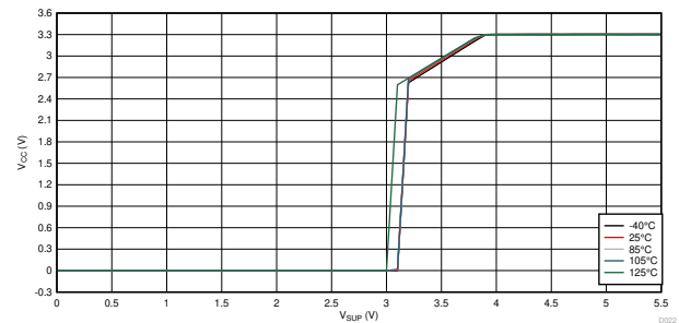
Figure 10-4. V_{CC} vs V_{SUP} Across Temperature
