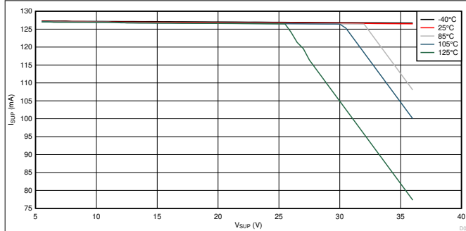
Figure 7-1. I_{SUP} vs V_{SUP} Across Temperature
