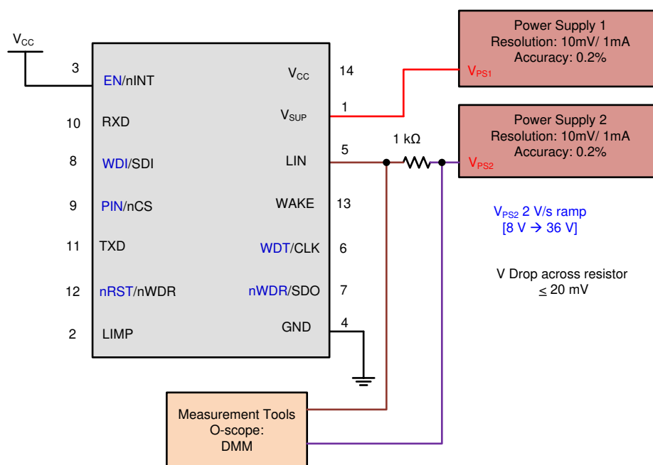
Figure 8-8. Test Circuit for I_{BUS\_PAS\_rec}
