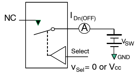
Figure 6. Off Leakage
