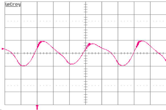
Figure 10. Output voltage ripple (20 mV/div.) at full rated load current into a resistive load with C_o = 10\ \mu\text{F} tantalum + 1\ \mu\text{F} ceramic and V_{in} = 48\ \text{V} . Time scale: 1\ \mu\text{s}/\text{div} .
