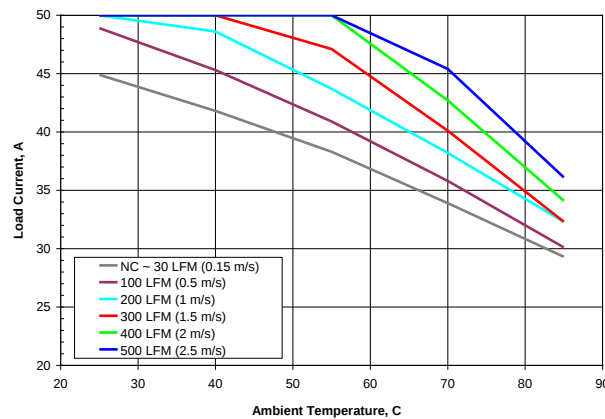
Figure 1. Available load current vs. ambient air temperature and airflow rates for SQE48T50012 converter mounted vertically with air flowing from pin 3 to pin 1, MOSFET temperature \leq 120^\circ\text{C} , V_{in} = 48\text{ V} . Note: NC – Natural convection
