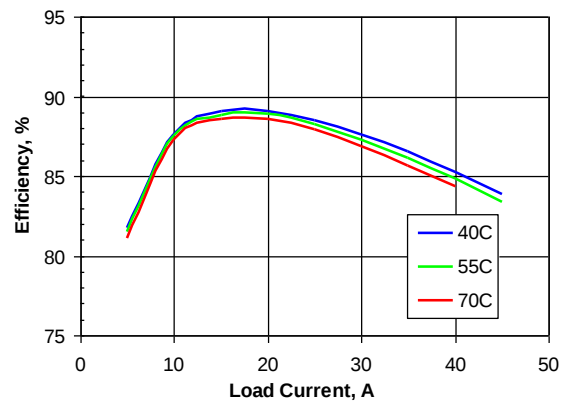
Figure 3. Efficiency vs. load current and ambient temperature for SQE48T50012 converter mounted vertically with V_{in}=48\text{V} and air flowing from pin 3 to pin 1 at 200LFM (1.0m/s).
