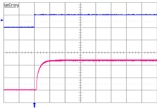
Figure 6. Turn-on transient at full rated load current (resistive) with no output capacitor at V_{in} = 48\text{ V} , triggered via ON/OFF pin. Top trace: ON/OFF signal (5 V/div.). Bottom trace: Output voltage (0.5 V/div.). Time scale: 5 ms/div.
