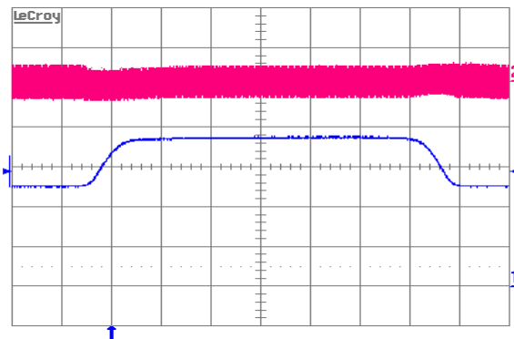
Figure 8. Output voltage response to load current step-change (25 A – 37.5 A – 25 A) at V_{in} = 48\text{ V} . Top trace: output voltage (20 mV/div.). Bottom trace: load current (10 A/div.). Current slew rate: 0.1 A/ \mu\text{s} . C_o = 1\text{ }\mu\text{F} ceramic. Time scale: 0.2 ms/div.
