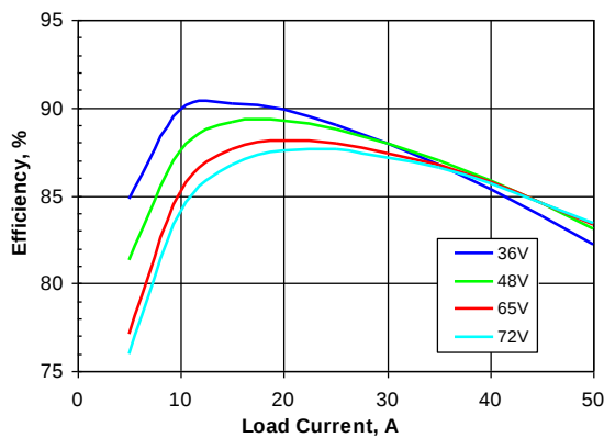
Figure 2. Efficiency vs. load current and input voltage for SQE48T50012 converter mounted vertically with air flowing from pin 3 to pin 1 at 300 LFM (1.5 m/s) and T_a=25^\circ\text{C} .
