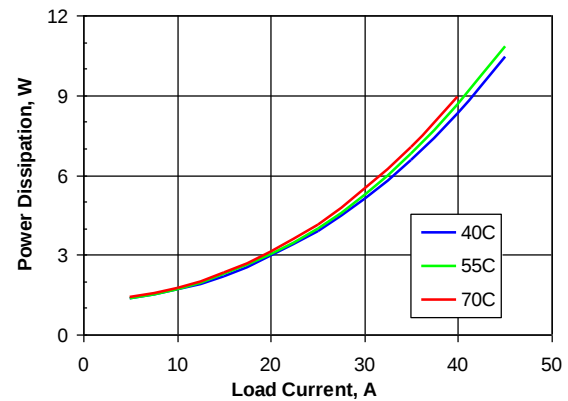
Figure 5. Power dissipation vs. load current and ambient temperature for SQE48T50012 converter mounted vertically with V_{in} = 48\text{ V} and air flowing from pin 3 to pin 1 at a rate of 200 LFM (1.0 m/s).
