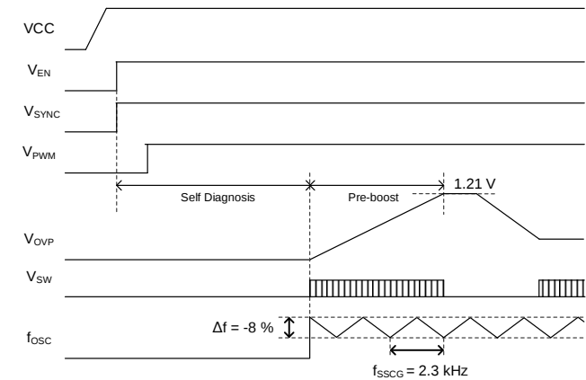
Figure 22. Spread Spectrum Function Timing Chart
