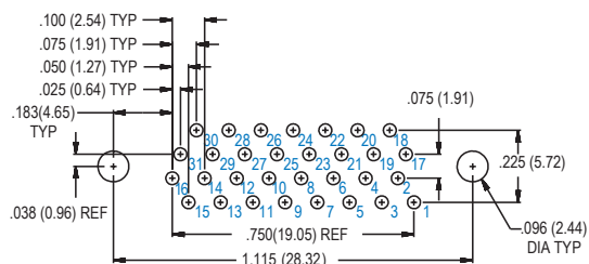
31 PIN
