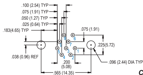
9 PIN
