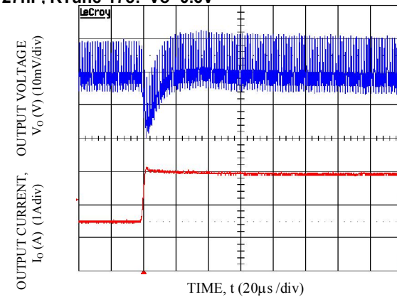
Transient Response to Dynamic Load Change from 50% to 100% at 12Vin, Cout-1x47uF+1x330uF, CTune-10nF & RTune-261. Vo=1.8V
