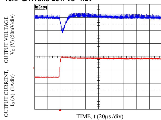
Transient Response to Dynamic Load Change from 50% to 100% at 12Vin, Cout-2x47uF, CTune-2700pF & RTune-261. Vo=2.5V
