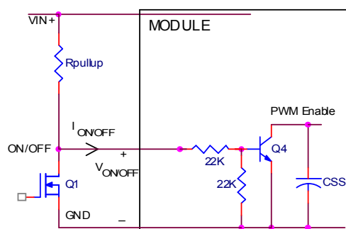
Circuit configuration for using negative On/Off logic.
