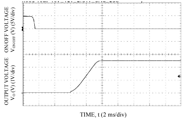
Start-up Using On/Off Voltage ( I_o = I_{o,max} ), V_o=2.5V
