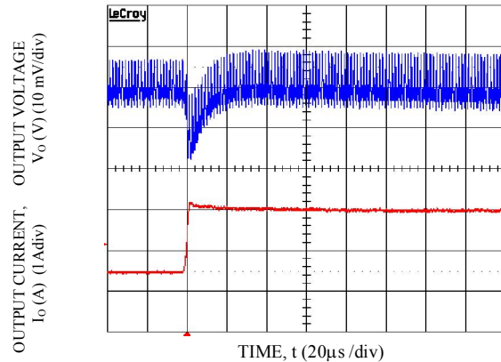
Transient Response to Dynamic Load Change from 50% to 100% at 12Vin, Cout-1x47uF+1x330uF, CTune-10nF & RTune-261. Vo=1.2V
