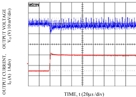
Transient Response to Dynamic Load Change from 50% to 100% at 8Vin, Cout-1x47uF+2x330uF, CTune-27nF, RTune-178. Vo=0.6V
