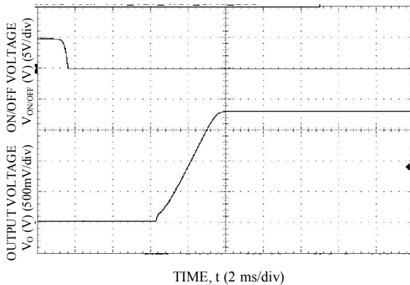
Start-up Using On/Off Voltage ( I_o = I_{o,max} ), V_o=1.8V
