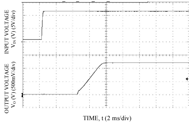
Start-up Using Input Voltage ( V_{IN} = 12V , I_O = I_{O,max} ), V_O = 1.2V
