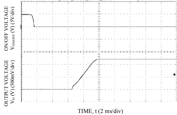
Start-up Using On/Off Voltage ( I_o = I_{o,max} ), V_o=1.2V
