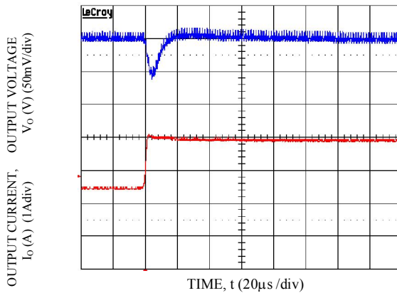
Transient Response to Dynamic Load Change from 50% to 100% at 12Vin, Cout-2x47uF, CTune-2200pF & RTune-261. Vo=3.3V
