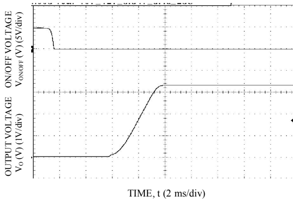
Start-up Using On/Off Voltage ( I_o = I_{o,max} ), V_o=3.3V
