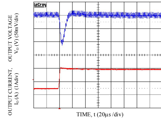
Transient Response to Dynamic Load Change from 50% to 100% at 12Vin, Cout-1x47uF, CTune-820pF & RTune-261. Vo=5V
