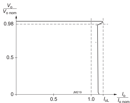
Fig. 6 Rectangular current limitation
