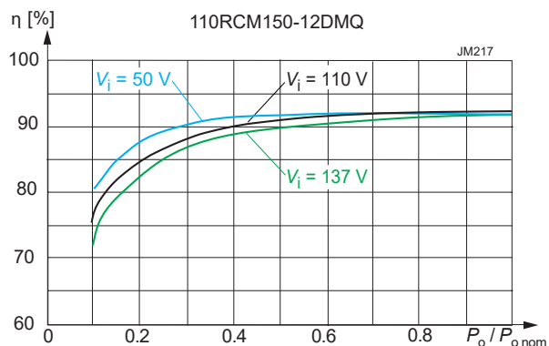
Fig. 3a Efficiency versus V_i and P_o (110RCM150-12DMQ)
