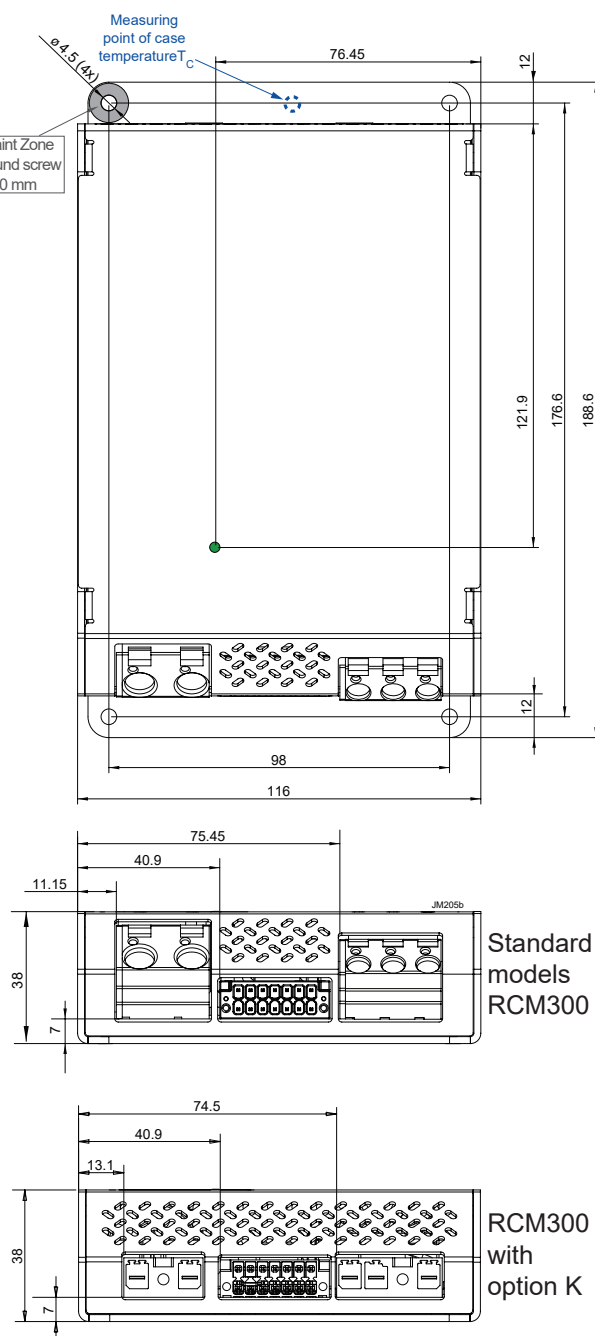
Fig. 12a Case of RCM300 (RCM02) weight approx. 820 g, Aluminum, EP-powder coated
