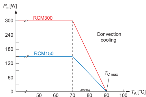
Fig. 5 Typical output power derating vs. temperature; vertical mounting position, free convection cooling
