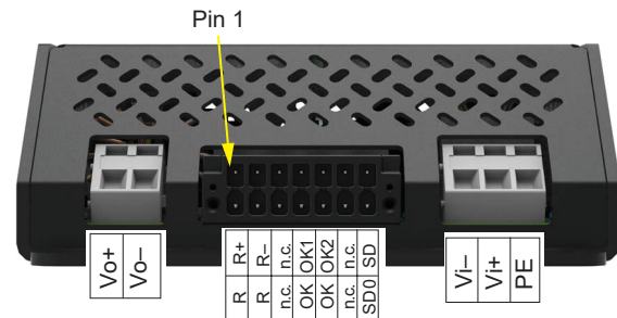
Fig. 13 Pin allocation of RCM150
