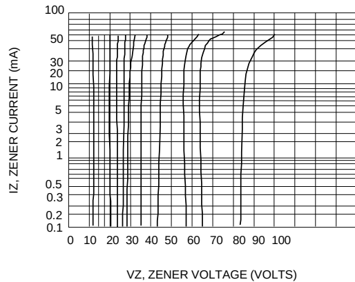
Fig. 3 BREAKDOWN CHARACTERISTICS (V Z = 12 - 82 V)
