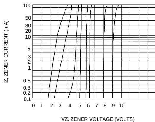
Fig. 2 BREAKDOWN CHARACTERISTICS (V Z = 3.9 - 10 V)
