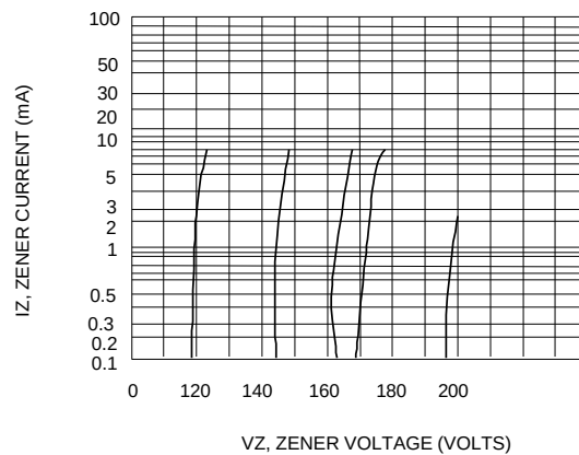
Fig. 4 BREAKDOWN CHARACTERISTICS (V Z = 100 - 200 V)
