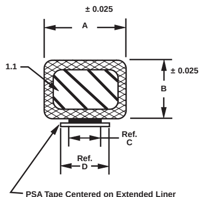
Figure 1. UltraSoft® Knit Rectangle
