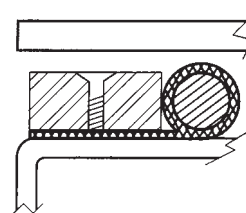
Elastomer Core with Hold Down Bar and Positive Stop
