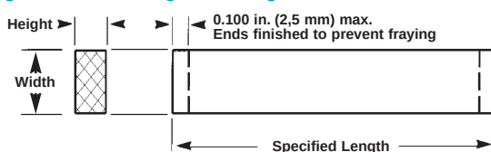
Figure 3. Cut-to-length Rectangular
