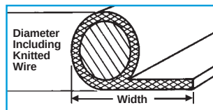
Single Fin with Sponge Elastomer
