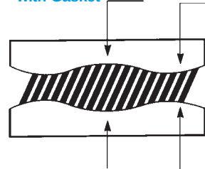
Figure 6b. Uneven Joint with Gasket
