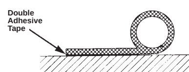
Adhesive Mounting
