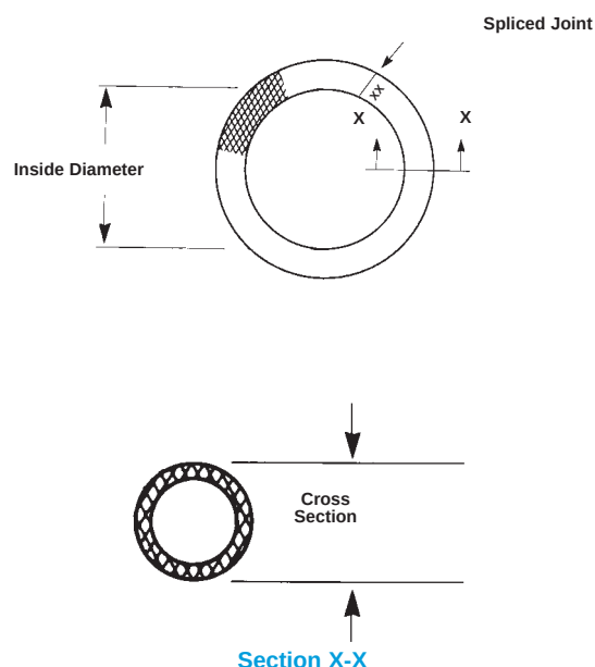
Figure 1. O-Ring Construction
