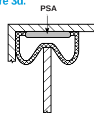
Partition with Knife-Edge Contact
