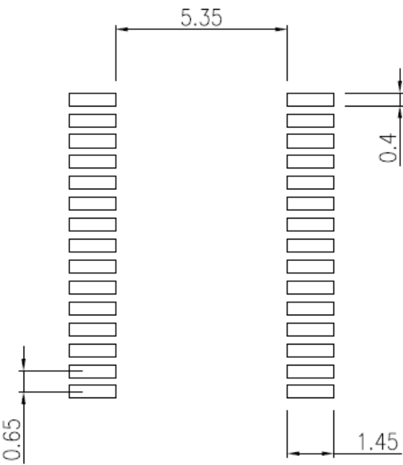
Figure 13.3 Land Pattern Dimensions for Reference only
