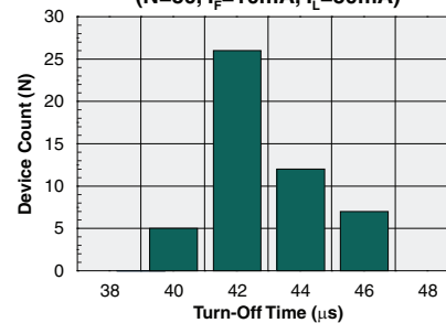
Turn-Off Time Distribution (N=50, I_F=10\text{mA} , I_L=50\text{mA} )
