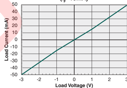
Typical Load Current vs. Load Voltage ( I_F=10mA )
