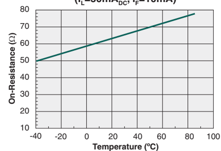
Typical On-Resistance vs. Temperature ( I_L=50mA_{DC} , I_F=10mA )
