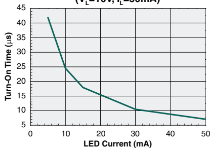
Typical Turn-On Time vs. LED Forward Current ( V_L=10\text{V} , I_L=50\text{mA} )
