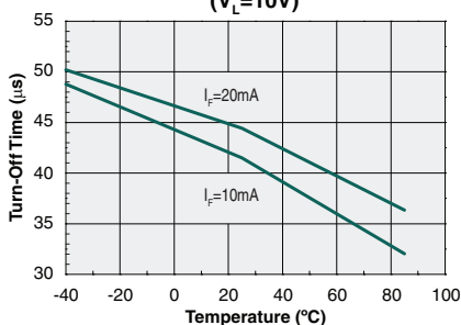
Typical Turn-Off Time vs. Temperature ( V_L=10V )
