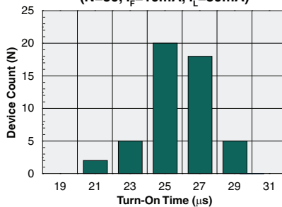
Turn-On Time Distribution (N=50, I_F=10\text{mA} , I_L=50\text{mA} )
