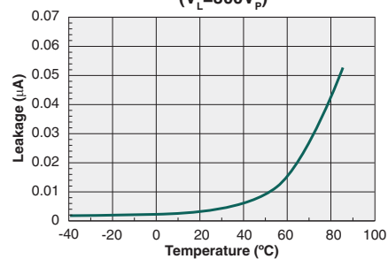
Typical Leakage vs. Temperature Measured across Pins 4&6 ( V_L=300V_P )
