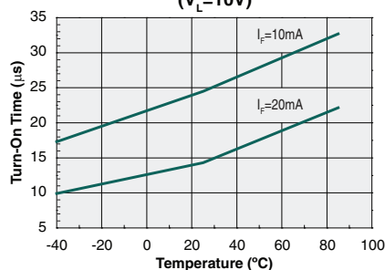
Typical Turn-On Time vs. Temperature ( V_L=10V )
