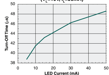
Typical Turn-Off Time vs. LED Forward Current ( V_L=10\text{V} , I_L=50\text{mA} )
