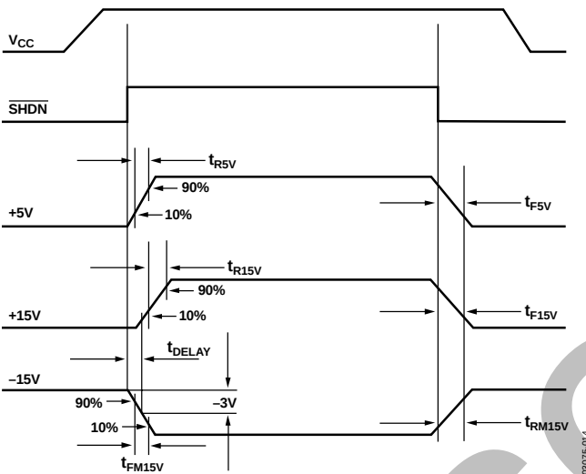
Figure 14. Power Sequence
