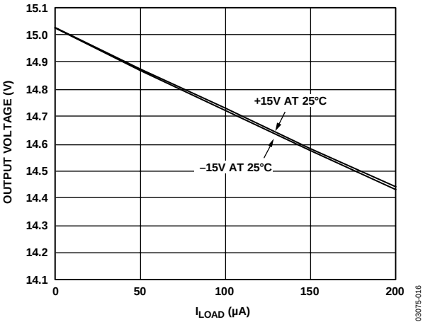
Figure 16. +15 V/-15 V Output Voltage vs. Load Current, Typical Configuration
