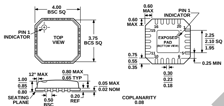
COMPLIANT TO JEDEC STANDARDS MO-220-VGGD-1 Figure 19. 20-Lead Lead Frame Chip Scale Package [LFCSP_VQ] 4 mm × 4 mm Body, Very Thin Quad (CP-20-1) Dimensions shown in millimeters
