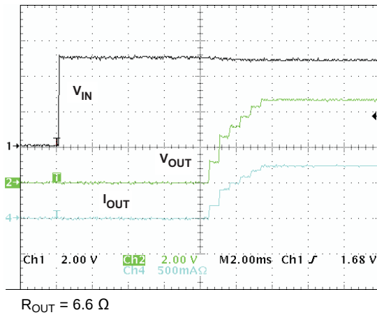
Figure 12. Normal Power-On Showing Soft-Start
