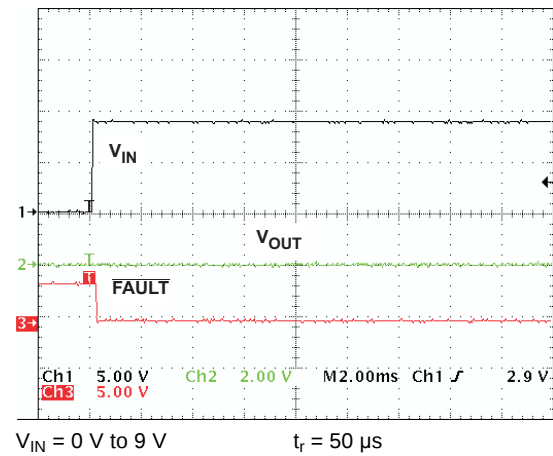
Figure 13. OVP at Power-On
