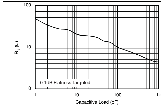
Figure 29. Recommended R_S vs Capacitive Load
